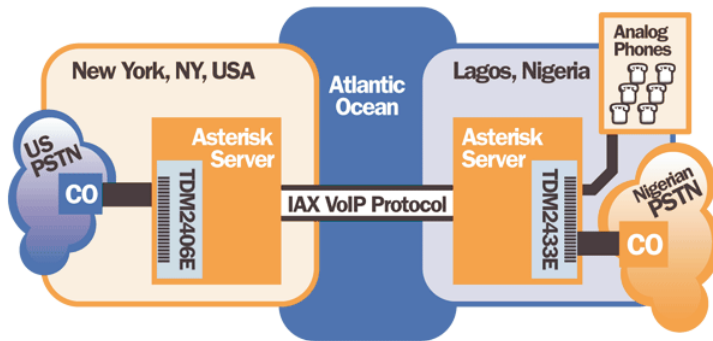
Figure 3: Sample Application - Toll-bypass
