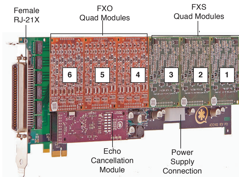
Figure 6: AEX2400 Card (Model TDM2433E)
