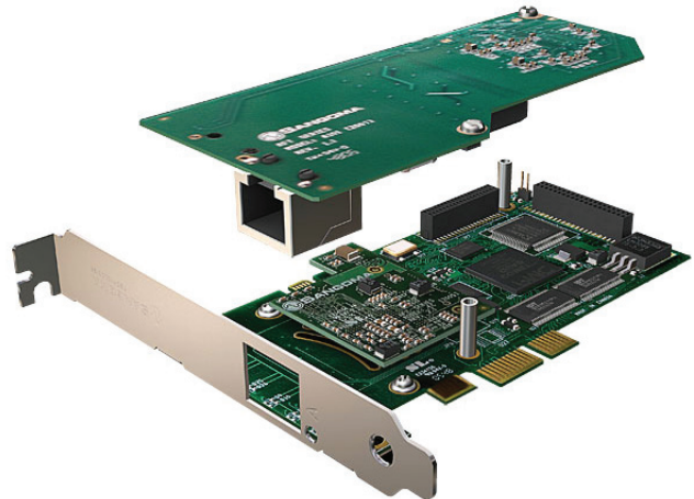
A101DE 1-port T1/E1/J1 shown with available Echo Cancellor and PCI-Express Interface.
